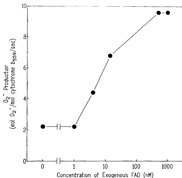
Fig. 3. Dependence of O_2^- production on exogenous FAD. Purified cytochrome b_{559} was reconstituted with a mixture of phosphatidylcholine, type II-S and phosphatidic acid, in the absence of exogenous FAD, and O_2^- production was assayed, essentially as described in the legend of Fig. 2, in the presence of various concentrations of FAD added to the assay medium
